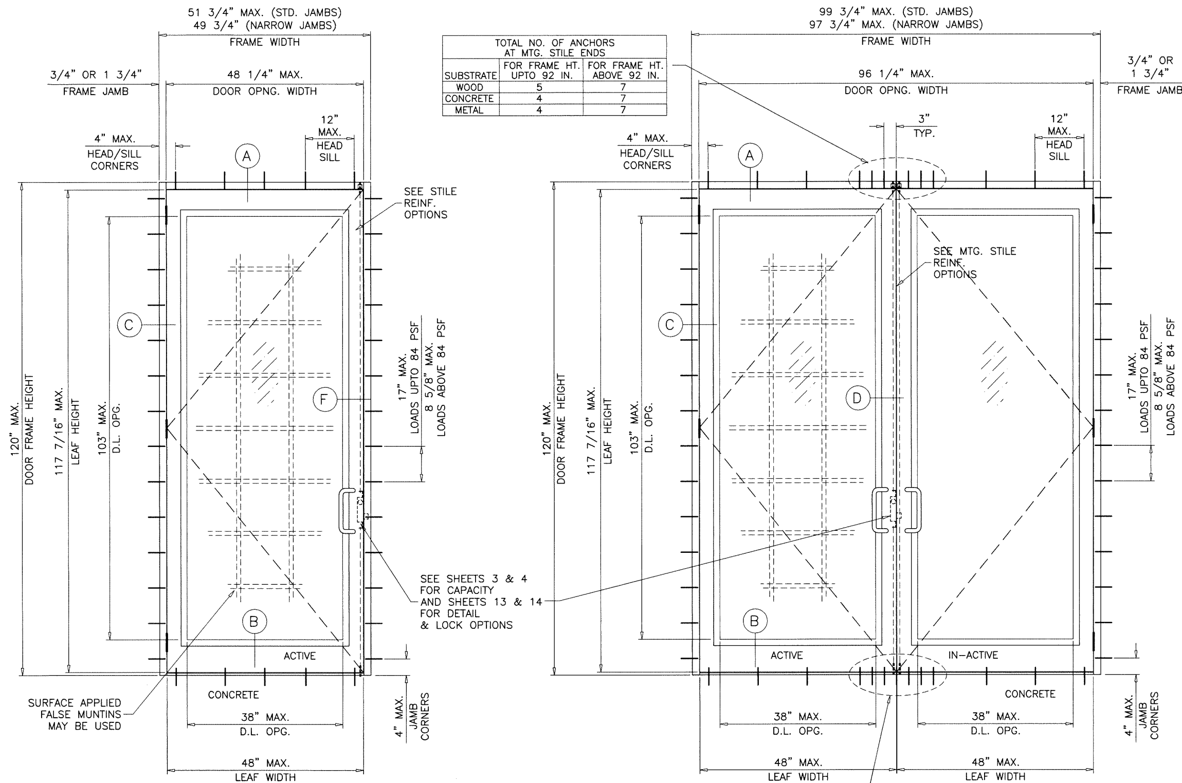
TYPICAL ELEVATIONS
